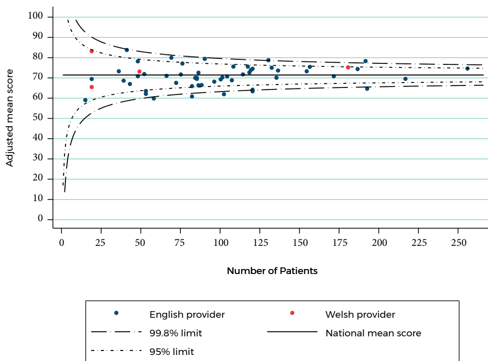
Figure 11. Adjusted funnel plot for the mean urinary incontinence score after radical prostatectomy by surgical centres in England and Wales.
