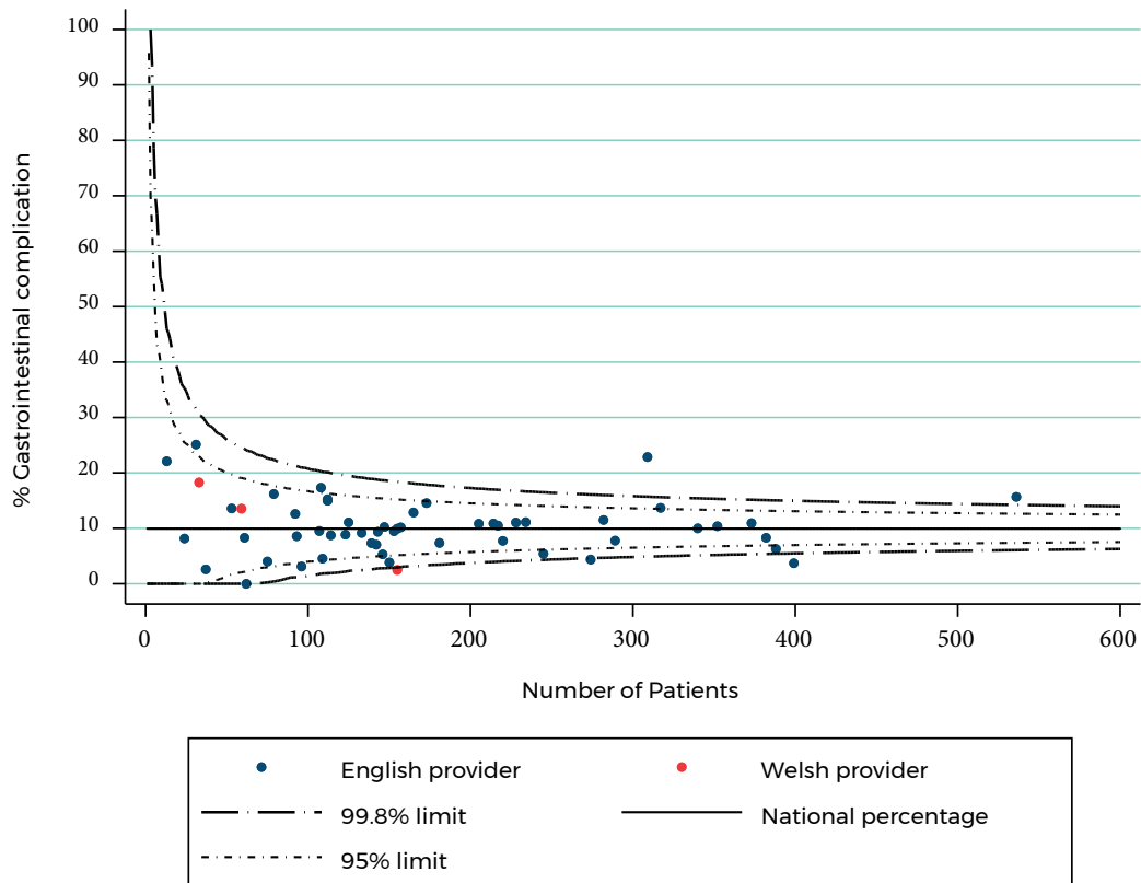
Figure 6. Adjusted funnel plot for the proportion of patients who experienced a severe gastrointestinal complication with 2 years of radical radiotherapy by radiotherapy centres in England and Wales.
