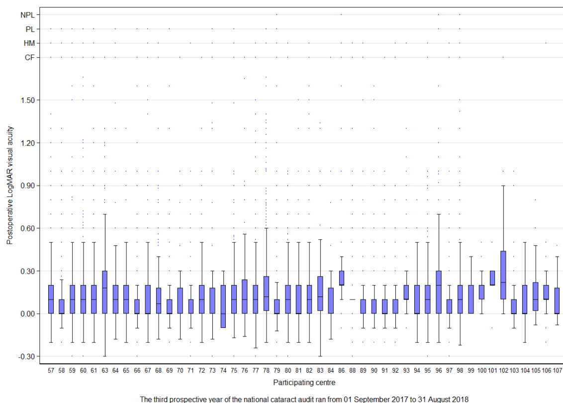
Figure 3b: Box and whisker plots of postoperative VA by participating centre Centres joining in audit year 2 (Centres 57 – 87) and audit year 3 (Centres 88 – 108)
