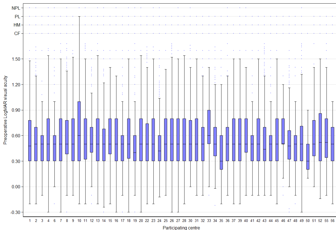
Figure 1a: Box and whisker plots of preoperative VA by participating centre Established centres with data in the first year audit report (Centres 1 – 56)
