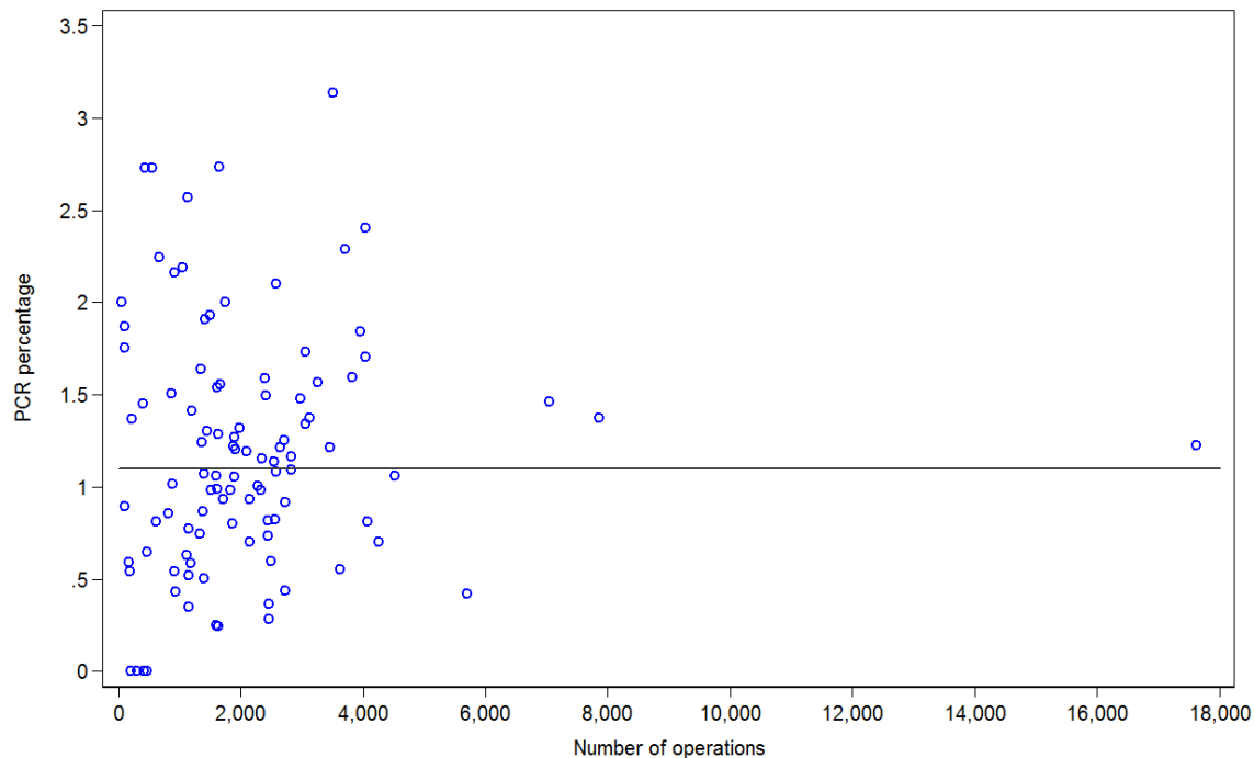
Figure 5: Unadjusted for case complexity PCR funnel plot for participating centres
