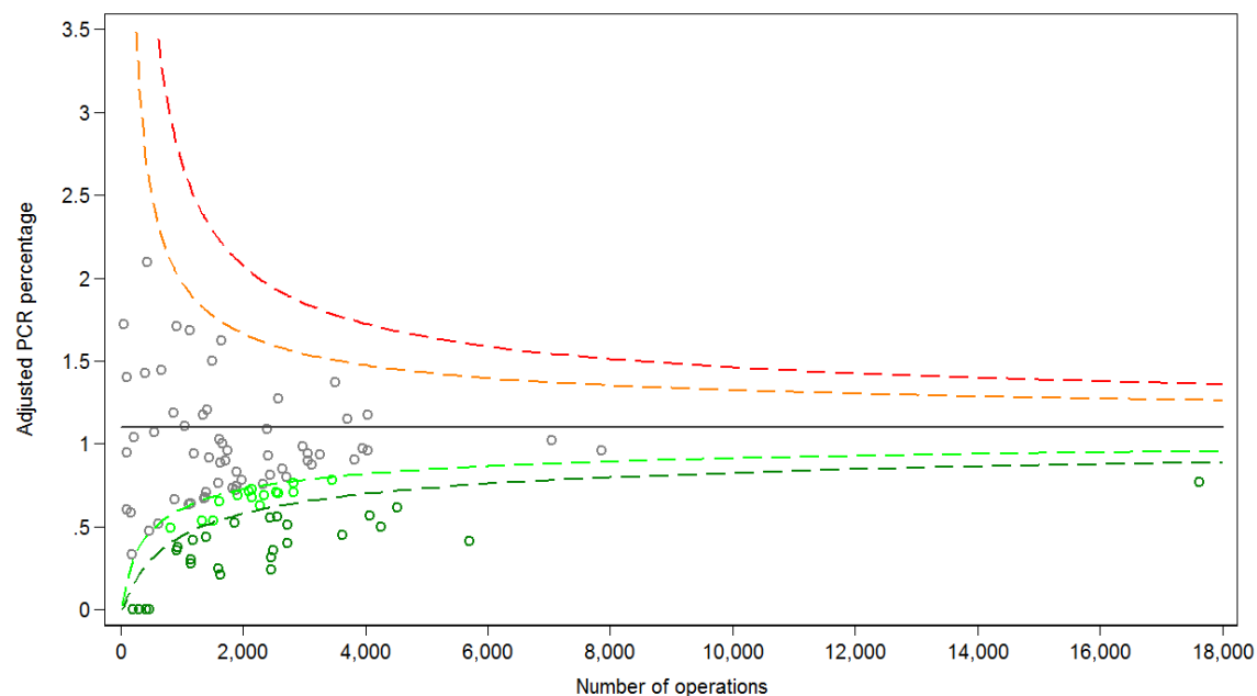
Figure 6: Adjusted for case complexity PCR funnel plot for participating centres
