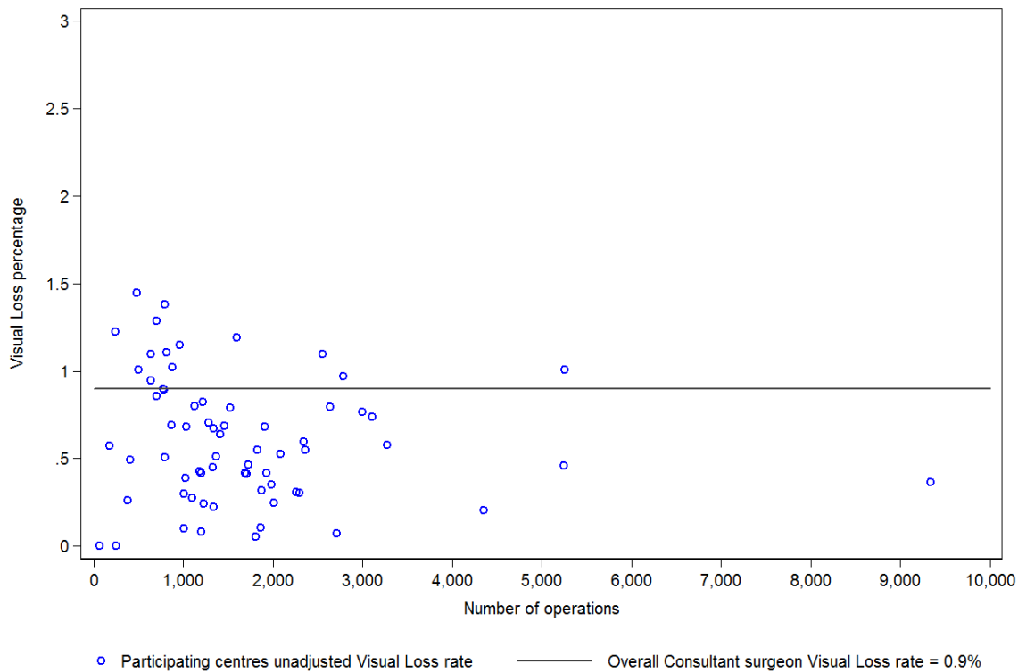
Figure 7: Unadjusted for case complexity VA Loss funnel plot for participating centres
